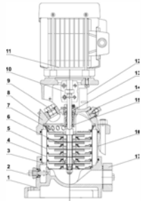
MODEL: TVR1 (2.3.4.5)
