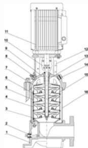
MODEL: TVR10 (15.20)
