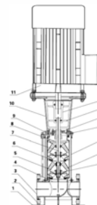
MODEL: TVR120 (150.200)
