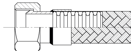
Female Swivel Nut
