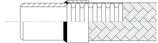
Bevelled End
