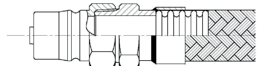
Male Nipple + -Quick Release Coupling-Male
