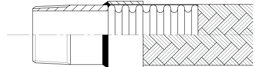
Thread End
