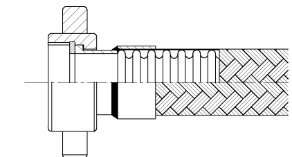
Pinlug Swivel Nut
