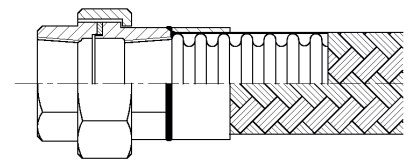
Union (Butt Welded)
