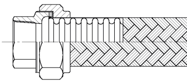
Female Union (Socket Welded)
