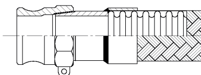
Thread End + Camlock Part A
