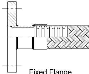
Fixed Flange
