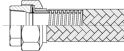
Union (Non Welding)
