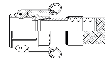
Thread End + Camlock Part D
