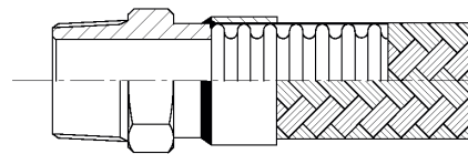
Male Nipple
