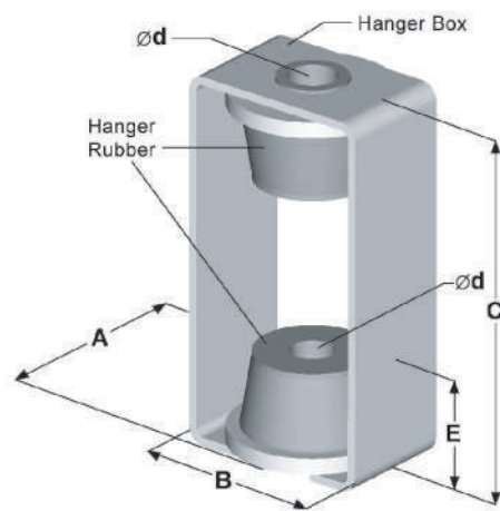
PTH-GG-80, 120, 150, 200, 300, 450
