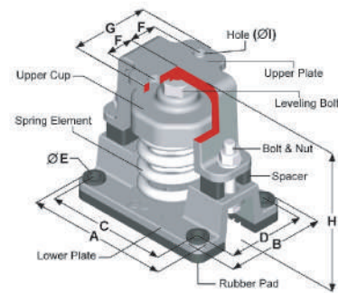
PTM-D- 451, 601, 826 , 1101 , 1401 PTM-D2-176, 246, 351, 526, 751, 1051
