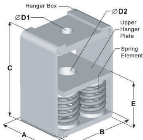
PTH-S-xxx4, PTH-S2-xxx4
